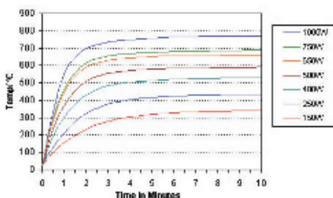
Heat Up Graph for PQR / PQP / PQC models
