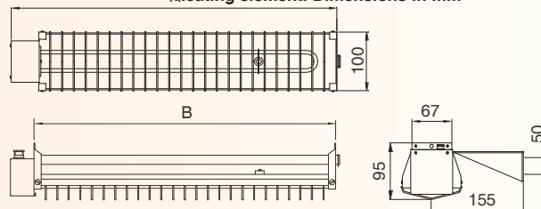
Heating element. Dimensions in mm
