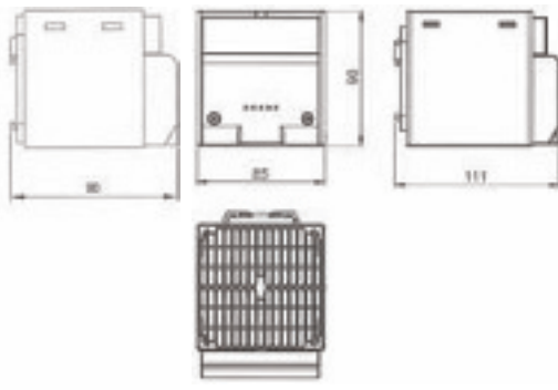
Dimensions model CS 028
