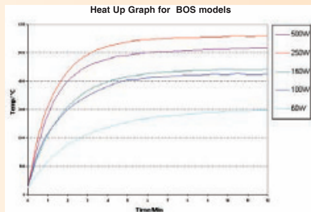
Heated side
